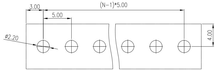
PCB LAYOUT
