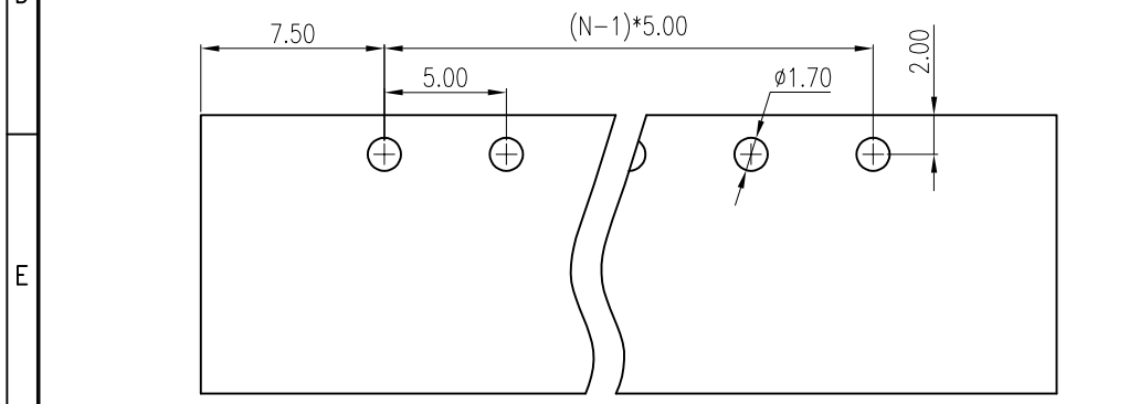
PCB LAYOUT
