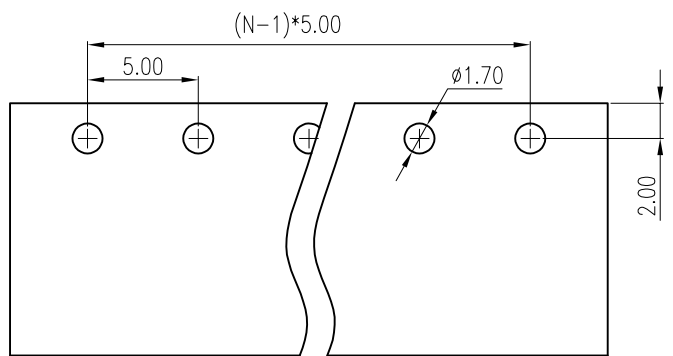
PCB LAYOUT
