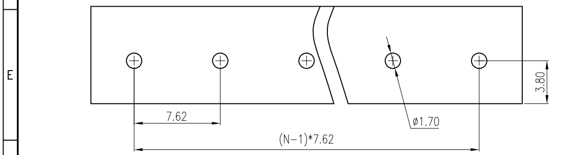
PCB LAYOUT
